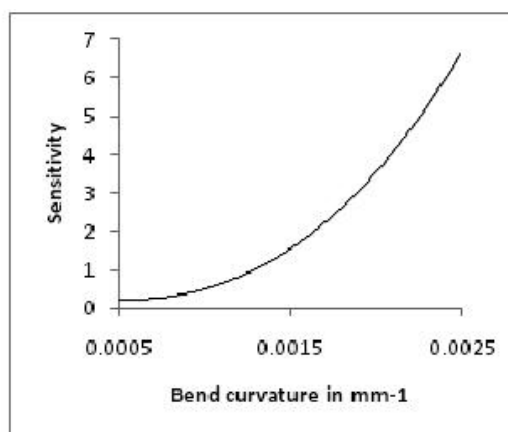
Fig. 5 Improvement in sensitivity with bending curvature
