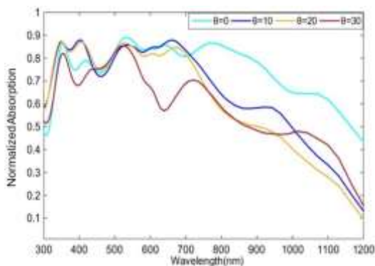
Fig. 11. Absorption spectra at different incidence angles.
