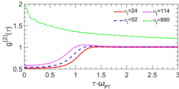
Fig. 2. The second-order coherence g^{(2)}(\tau) versus \tau \omega_{PT} for two-photon wave packet transmitted through the bilayer structure for \alpha_1=24, 52, 114, and 890 .
