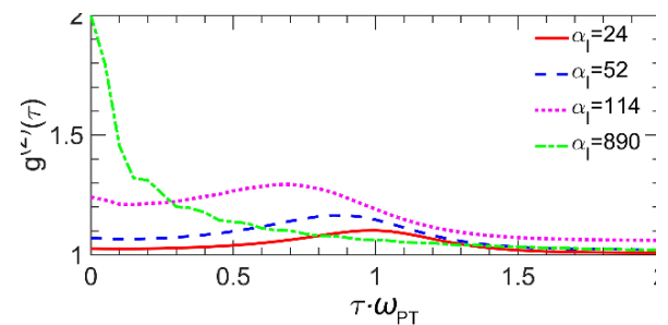
Fig. 3. The second-order coherence g^{(2)}(\tau) versus \tau \omega_{PT} for coherent state transmitted through the bilayer structure for \alpha_1=24, 52, 114, and 890 .
