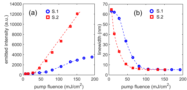
Fig. 13. Comparison between plots of: (a) maximum emitted intensity in arbitrary units, and (b) linewidth versus the pump fluence corresponding to the samples S1 and S2 at the excitation position P2.
