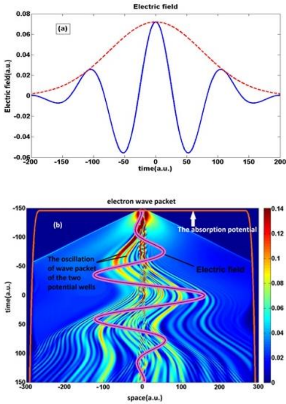
Fig. 1. (a). One color laser field (blue solid line) with a Gaussian envelope (red dashed line) and (b). Its corresponding wave packet for \tau = 3 fs . The orange line determines the absorption potential. The pink line shows electric field.
