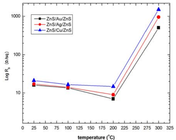
Fig. 2 The sheet resistance of ZMZ nanomultilayer films as a function of annealing temperature.
