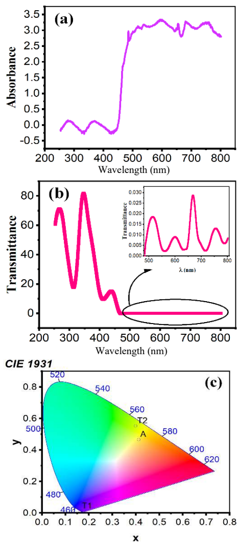
Fig. 4. (a) Absorption spectra, (b) transmittance spectra, and (c) extracted CIE colorimetry diagram of the sample.
