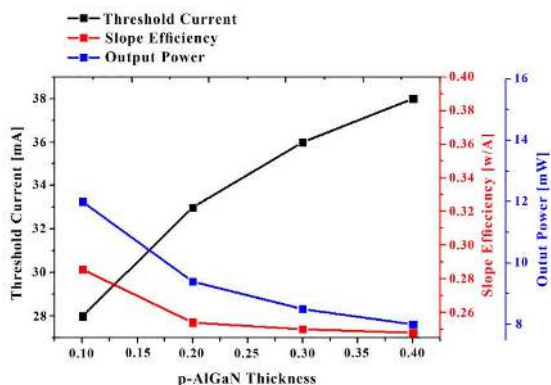
Fig. 8. Threshold current, output power and slope efficiency of LDs with different p-AlGaIn thicknesses.
