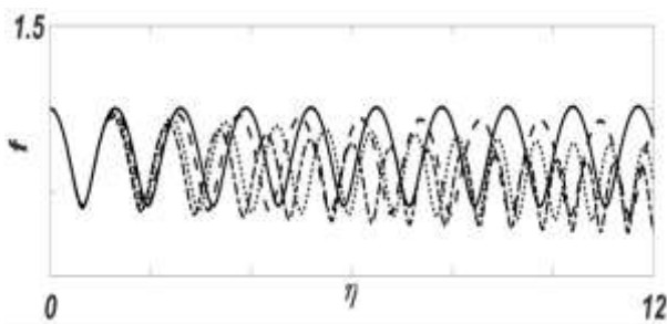
Fig. 8. Variation of beam width parameter, f , respect to propagation distance, \eta , at T_{e06} = 175keV for \alpha A_{00}^2 = 0.8eV , r_0 = 20\mu m , n_0 = 2.4 \times 10^{18} cm^{-3} , \omega = 6.28 \times 10^{14} s^{-1} .
