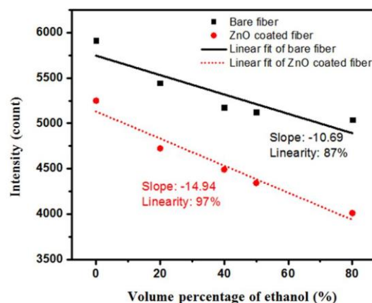
Fig. 6. Output intensity variation against ethanol concentration.
