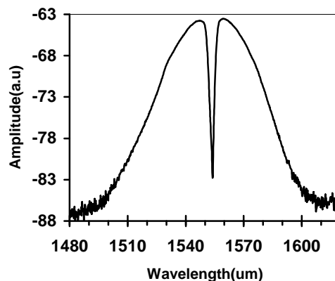
Fig. 3 Frequency response of a 1-D grating structure.
