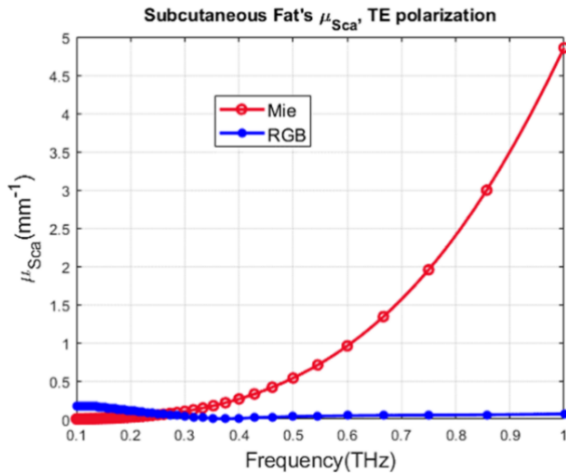
Fig. 1. Scattering coefficient in two conditions of air-enclosed (Mie) and tissue-enclosed (RGB) for TE Polarization.
