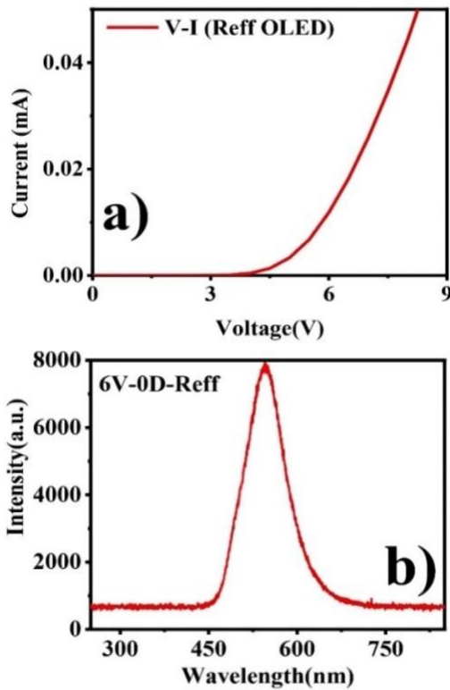
Fig. 2. a) I-V curve and b) the electroluminescence spectrum of the reference OLED.
