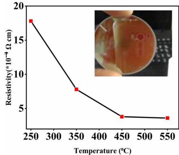
Fig. 5. Sheet resistance vs. annealing temperature (250–550 °C).
