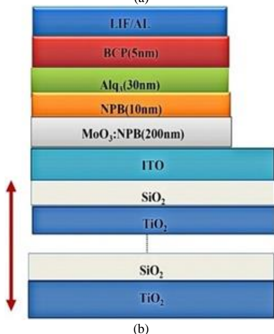
Fig. 7. a) Current density–voltage characteristic and the emission color of the 240 nm microcavity b) Schematic structure of the OLED in a DBR/Al-cathode micricavity.
