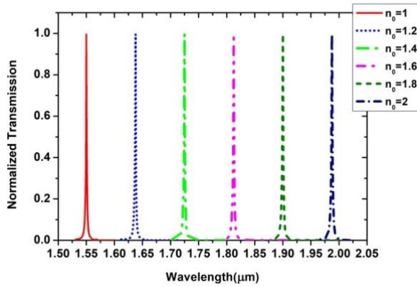
Fig. 14 Normalized transmission spectrum at forward dropping port C for varying background index ( n_0 ) of all holes for RI change from 1 to 2.
