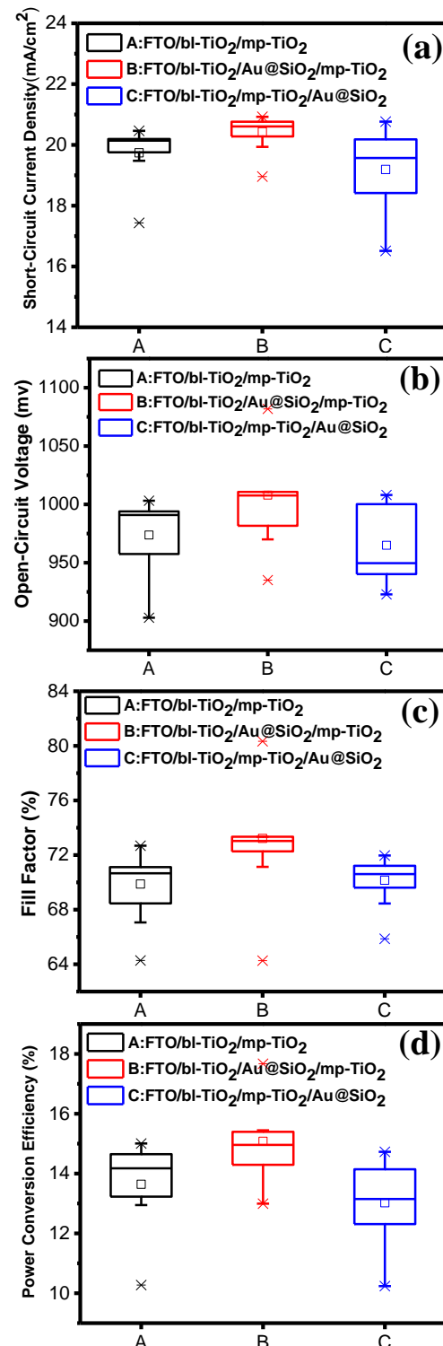
Fig. 7. Statistics parameters for the photovoltaic performance for 20 cells using different concentration of Au@SiO 2 (a) J sc , (b) V oc , (c) FF, (d) PCE. A:FTO/bl-TiO 2 /mp-TiO 2 , B:FTO/bl-TiO 2 /Au@SiO 2 /mp-TiO 2 , C:FTO/bl-TiO 2 /mp-TiO 2 /Au@SiO 2 .
