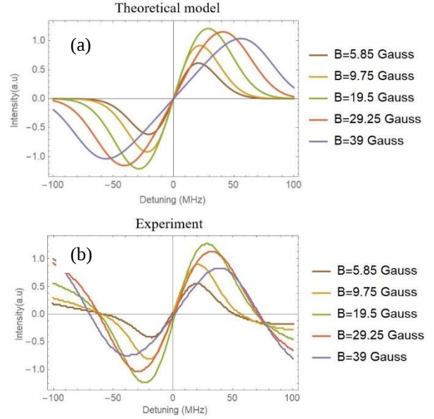
Fig. 6. The sub-Doppler error signal for different magnetic fields, (a) theoretical result, (b) experimental result.
