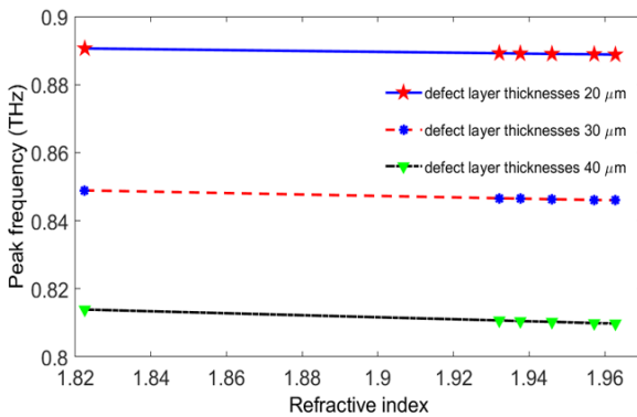
Fig. 10. The peak frequency of the defect modes of the 1D-PC-based biosensor with the structure (AB)^5D(AB)^5 versus the refractive index, n , of the analyte cancer cells for different thicknesses of the defect layer. The other parameters used here are the same as in Fig. 3.
