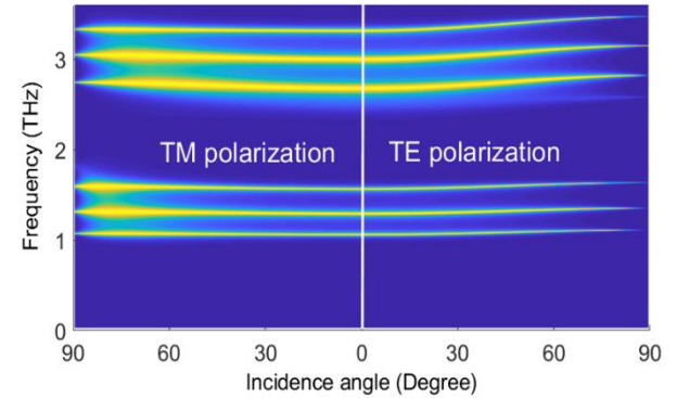
Fig. 2. The transmittance of the 1D-PC with the structure (AB)^5 in the plane (f, \theta) . Here, d_A = 5 \mu\text{m} , d_{0B} = 20 \mu\text{m} , T = 4.2 \text{ K} , and P = 1 \text{ atm} .
