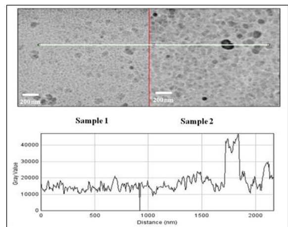
Fig. 6. The plot profile of two NCD thin films under side-by-side FESEM pictures for a straight line show the distance against the gray value in the case of samples 1 and 2.
