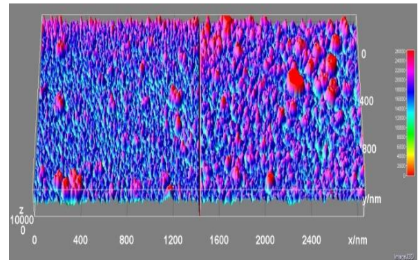
Fig. 5. The 3D view for FESEM images of sample 1 and 2. Two NCD thin films have been inserted to one side-by-side image.
