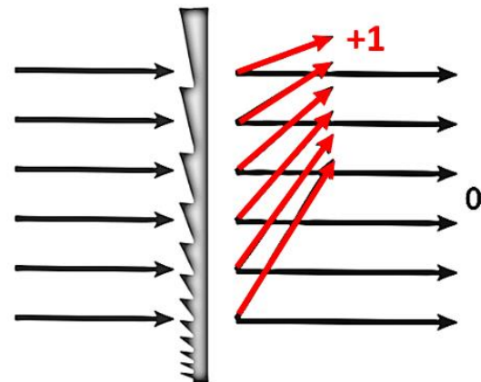
Fig. 3. Zero and first order diffraction of a chirped grating as far and near focal points, respectively.
