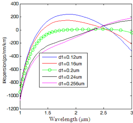
Fig. 3. Effect of Chalcogenide holes diameter on dispersion profile.
