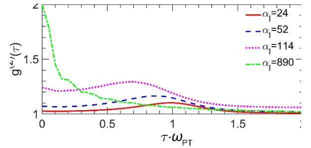
Fig. 3. The second-order coherence g^{(2)}(\tau) versus \tau\omega_{PT} for coherent state transmitted through the bilayer structure for \alpha_l=24, 52, 114 , and 890.
