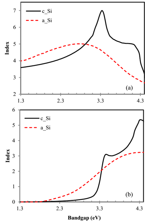
Fig. 2. The correlation between bandgap and optical properties for different layers of NWSCs, a) real part and b) imaginary part of refractive indices.
