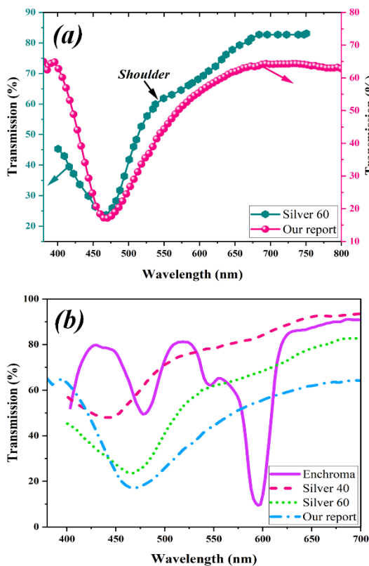
Fig. 4. (a) transmission spectra of the proposed plasmonic glasses in comparison with the transmission spectra of the reported plasmonic contact lens based on silver NPs [19], and (b) transmission spectra of the fabricated plasmonic glasses in comparison with the commercial Enchroma glasses, and plasmonic contact lenses based on Ag NPs [19].
