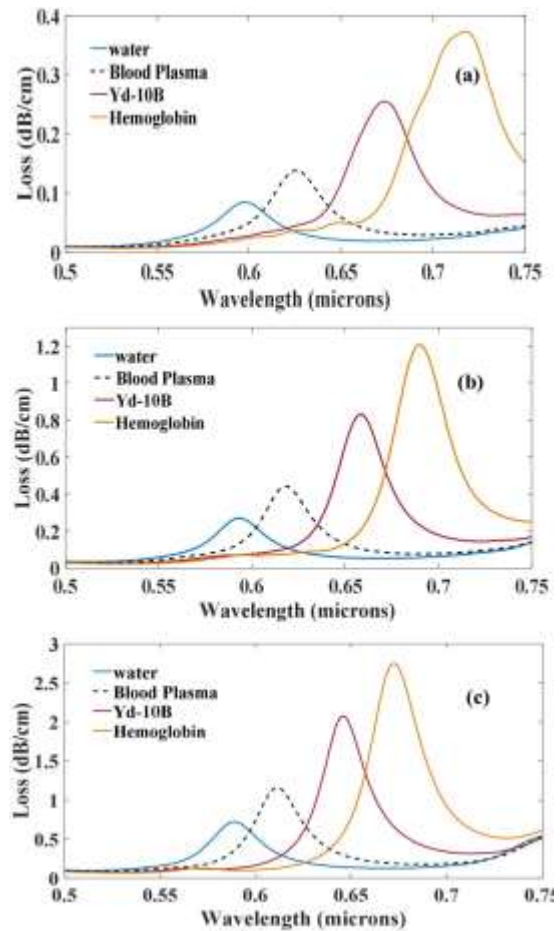
Fig. 6. The confinement loss spectra with different sensing layers and different pitch sizes \Lambda = (a) 1.9\mu\text{m} (b) 2\mu\text{m} (c) 2.1\mu\text{m} . The other parameters are d = 1.4\mu\text{m} , and d_{\text{Au}} = 45\text{nm} .
