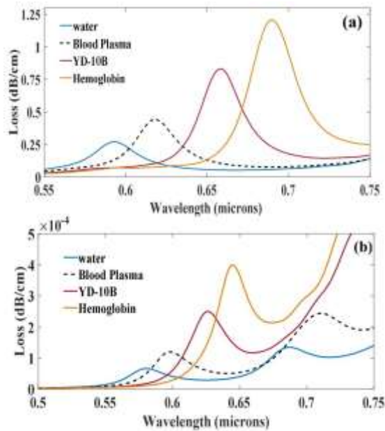
Fig. 5. The confinement loss as a function of the wavelength for different sensing layers and different hole diameters d = (a) 1.4\mu\text{m} and (b) 1.8\mu\text{m} . The other parameters are \Lambda = 2\mu\text{m} , and d_{\text{Au}} = 45\text{nm} .
