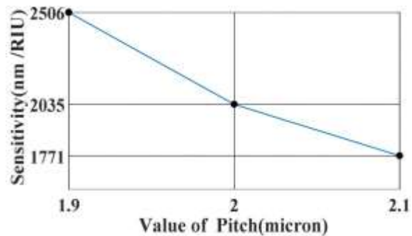
Fig. 9 Variation of the sensitivity in terms of the pitch size with d_{\text{Au}} = 45\text{nm} and d = 1.4\mu\text{m} .
