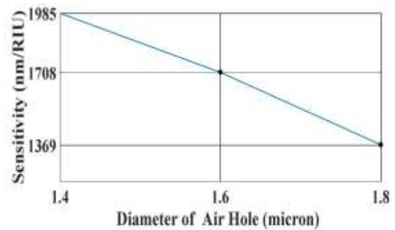
Fig. 8 Variation of the sensitivity in terms of the hole diameter with \Lambda = 2\mu\text{m} and d_{\text{Au}} = 45\text{nm} .
