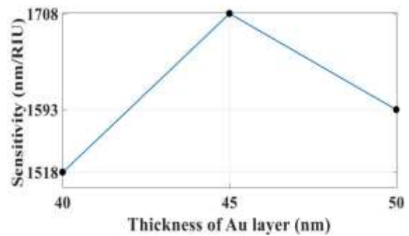
Fig. 7 Variation of the sensitivity in terms of the thickness of the Au layer with \Lambda = 2\mu\text{m} and d = 1.6\mu\text{m} .
