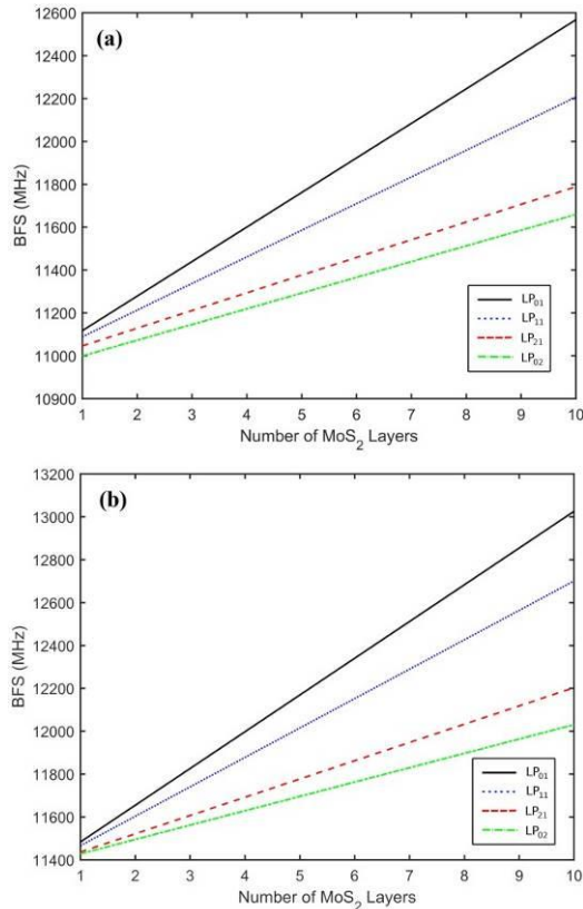
Fig. 8. Investigation of the effect of different layers \text{MoS}_2 on the BFS as a function of temperature and strain for 4 modes at (a) 100 °C and (b) 8000 \mu\epsilon .
