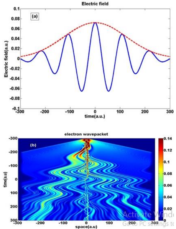
Fig. 2. (a). One color laser field (blue solid line) with a Gaussian envelope (red dashed line) and (b). Its corresponding wave packet for \tau = 5fs .
