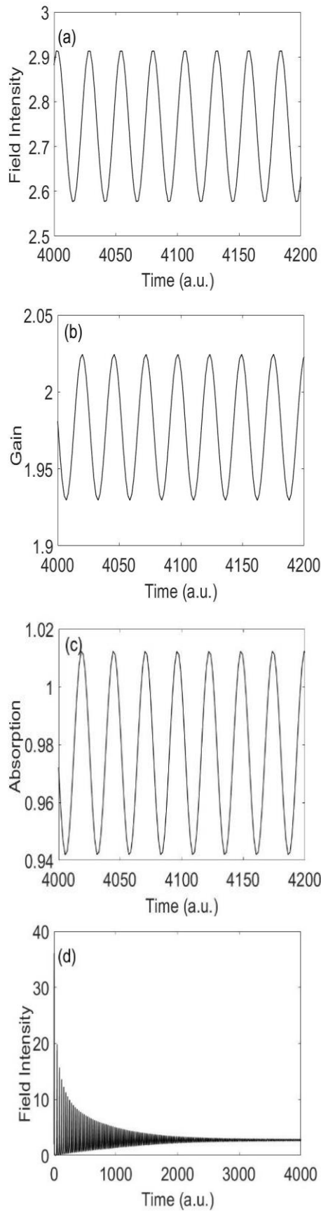
Fig. 3. Time evolution diagram of output field intensity, absorption and gain for a single laser in the presence of laser field intensity for numerical values: ( \gamma=0.04 , A=5.6 , B=5.8 , and \alpha=1.8 ).
