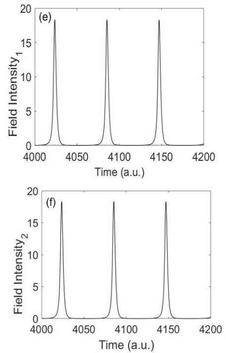
Fig. 5. Time evolution of absorption, Q and gain (G) and laser field intensity (I) in terms of time in two mutually coupled lasers with numerical values: ( \gamma=0.04 , A=5.6 , B=5.8 , \alpha=1.8 ).
