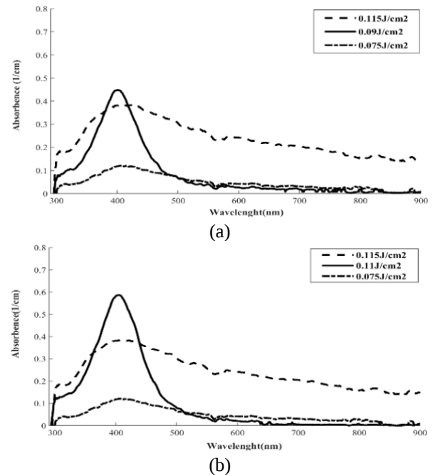
Fig. 3. UV-visible spectrum of Ag NPs at the number of the laser pulses at 900 and (a) three different laser energy densities: 0.115 \text{ J/cm}^2 and 0.09 \text{ J/cm}^2 and 0.075 \text{ J/cm}^2 (b) three different laser energy densities: 0.115 \text{ J/cm}^2 and 0.11 \text{ J/cm}^2 and 0.075 \text{ J/cm}^2 .
