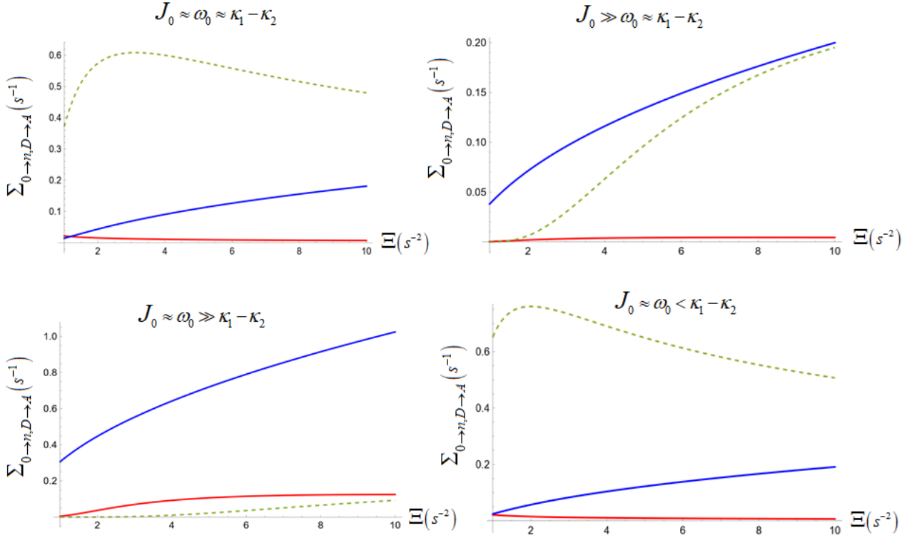
Fig. 3. Rate of inelastic tunneling is depicted for |0\rangle \rightarrow |1\rangle and |0\rangle \rightarrow |2\rangle excitation in vibrational mode of the quantum object for different amounts of J_0, \omega_0, \kappa_{1,2} against \Xi . The dashed line describes elastic rates where the quantum object is absent. Inelastic rates are dominant for larger values of J_0 and lower \Xi .
