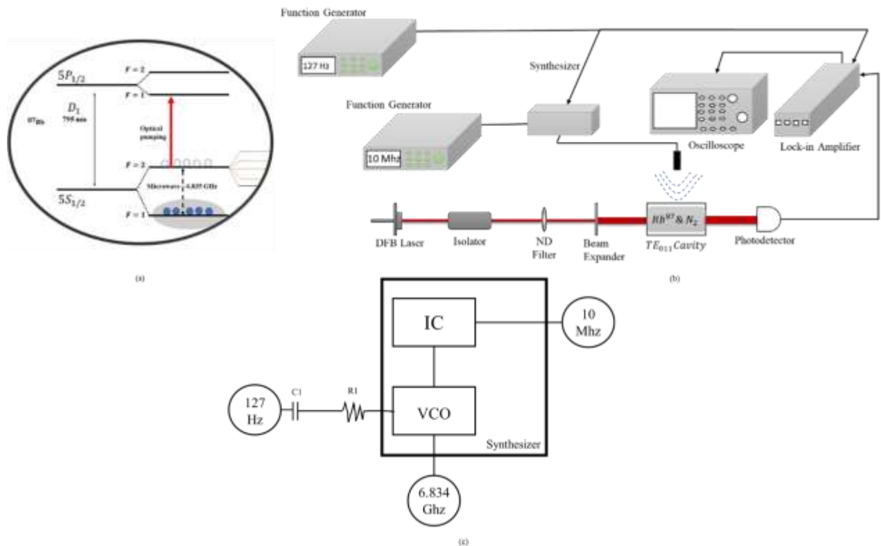
Fig. 1. (a) Fine and hyperfine structure of the \text{Rb}^{87} atom, illustrating the optical and microwave fields applied for double resonance. (b) Schematic diagram of the experimental setup used for the double resonance spectroscopy of \text{Rb}^{87} atoms, including the optical pumping configuration and the applied microwave field. (c) Block diagram of the frequency synthesizer, illustrating the main components responsible for generating, multiplying, and stabilizing the microwave output frequency.
