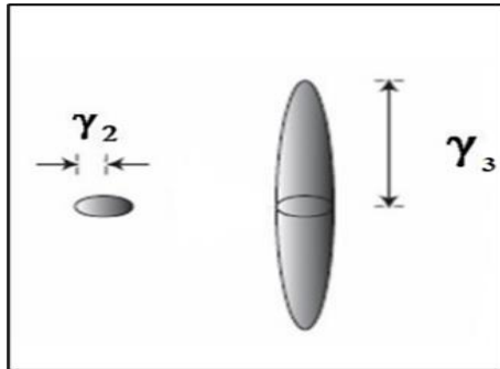
Fig. 3. A representation of ellipsoids.
