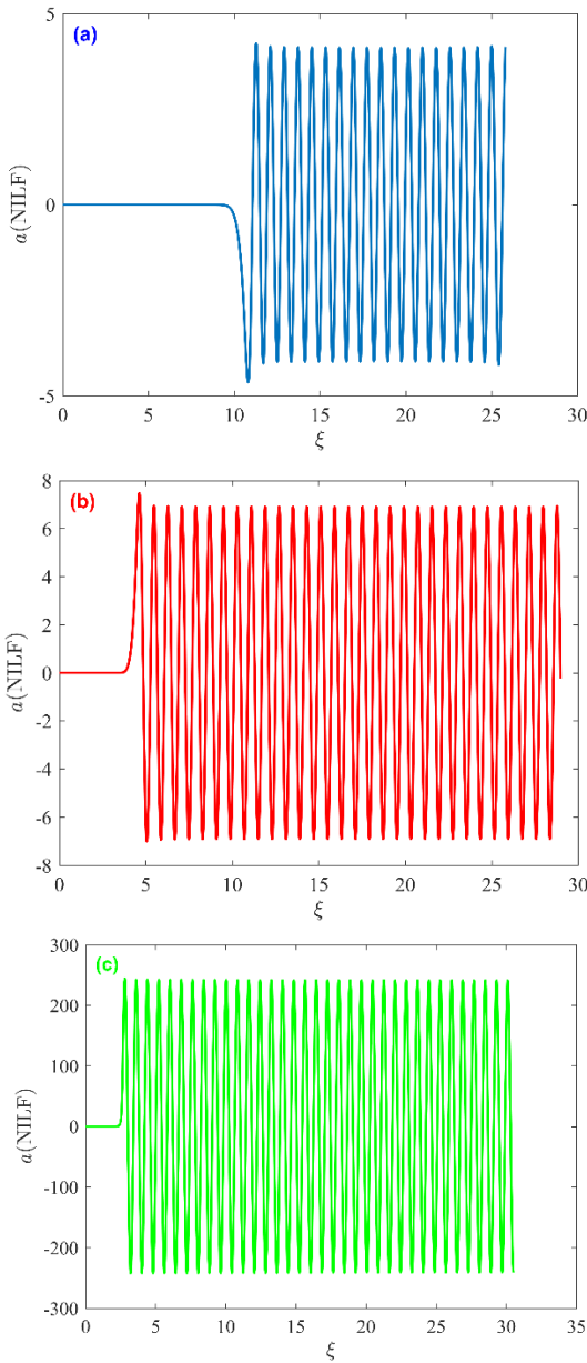
Fig. 3. Variation of NILF with \xi(\mu m) for (a) E_0 = 2.13 \times 10^{11} V/m , (b) E_0 = 4.28 \times 10^{11} V/m and (c) E_0 = 8.58 \times 10^{11} V/m for s=1 and r_0 = 32.94 \mu m
