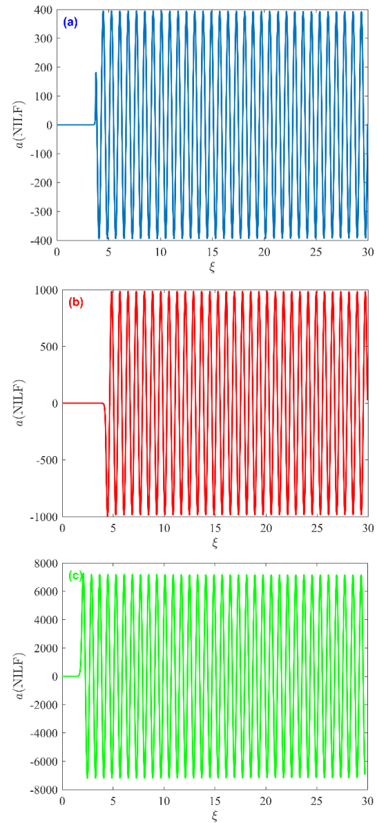
Fig. 4. Variation of NILF with \xi(\mu m) for (a) E_0 = 2.13 \times 10^{11} V/m , (b) E_0 = 4.28 \times 10^{11} V/m , and (c) E_0 = 8.58 \times 10^{11} V/m for s=2 and r_0 = 32.94 \mu m .
