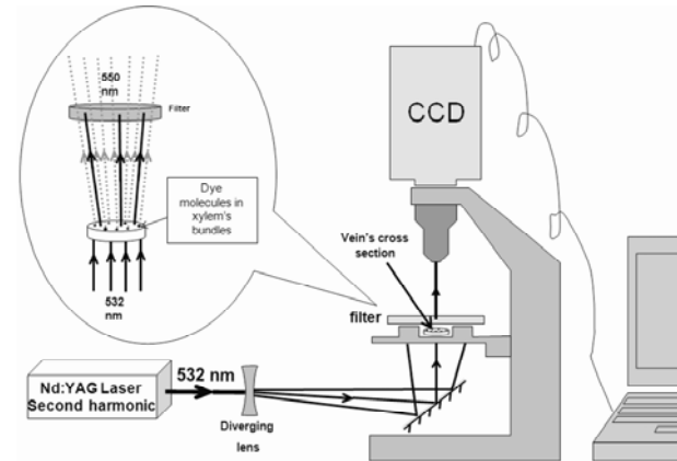
Fig. 9. Experimental setup to take a microscopical fluorescent photograph of vein's cross section
