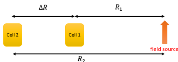
Fig. 1. Structure of magnetic gradiometer.
