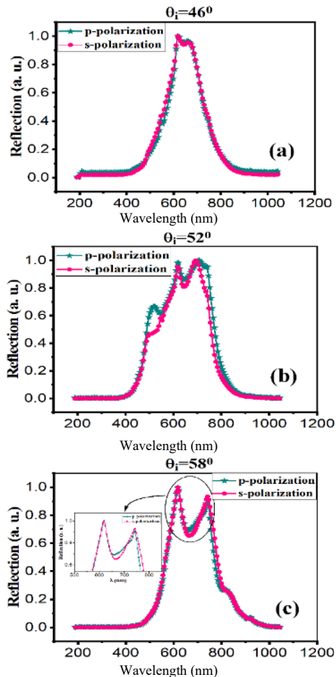
Fig. 5. Reflection spectra of the plasmonic structure under different incidence angles of (a) 46^\circ , (b) 52^\circ , and (c) 58^\circ for s and p-polarization.
