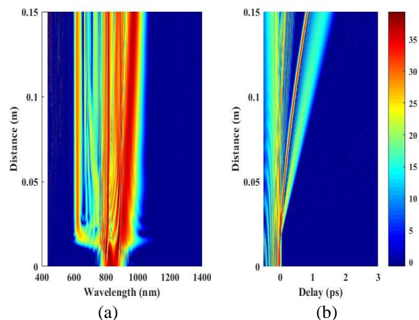
Fig. 2. Simulation results for the classical treatment of the SCG along the first 15 cm of a PCF fiber, when the stochastic term is not included. The spectra of light pulse versus wavelength are shown in (a), while the delay (+/-) with respect to the group velocity of the generated SCG is shown in (b).
