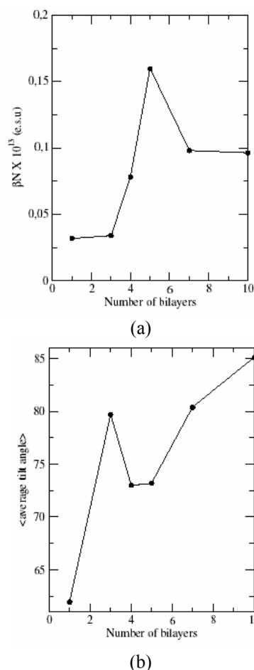
Fig. 6 Dependence of the hyperpolarizability (a) \beta and (b) tilt angle \theta of the DR1 moieties on the number of bi-layers as found by theoretical fitting of the data (see appendix).
