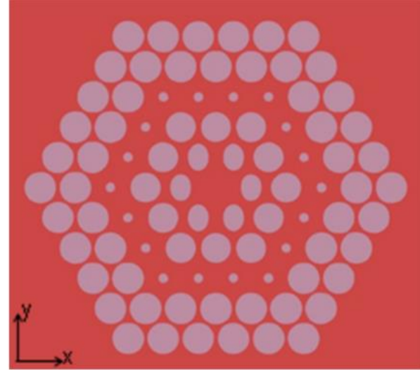
Fig. 1. The hexagonal lattice dispersion compensating fiber with elliptical holes.
