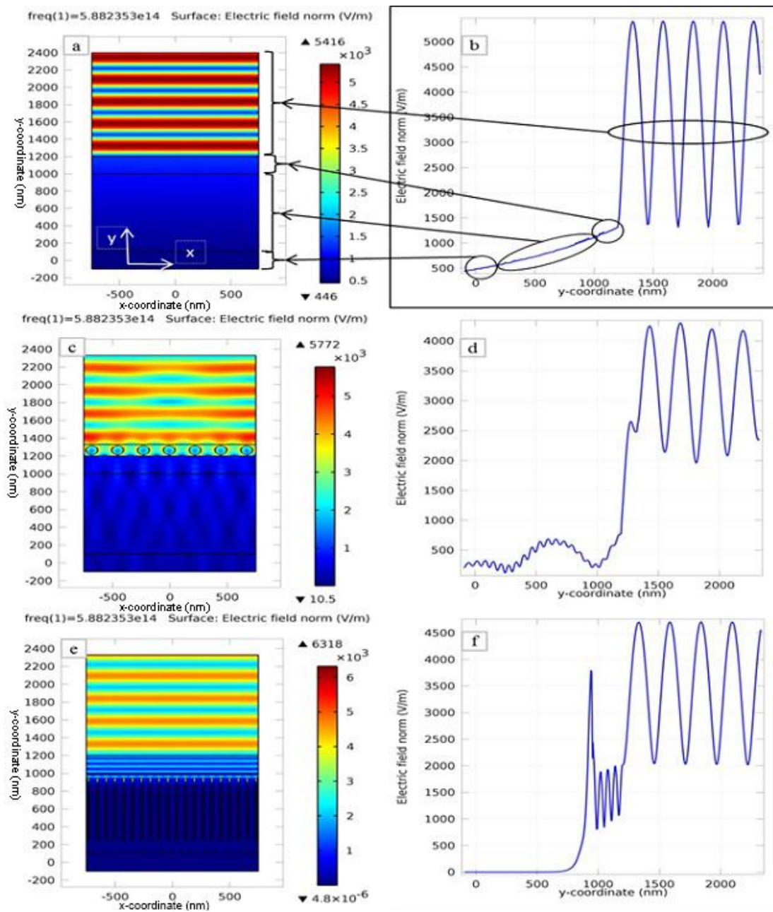
Fig. 2. Propagation of light in the (a) and (b) traditional structure, (c) and (d) improved structure with NPs in the addition region, (e) and (f) improved structure with NRs in the intrinsic area”.
