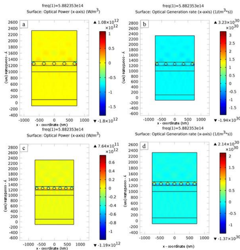
Fig. 5 NPs influence on optical power and generation rate, (a) NPs size alteration effect, (b) NPs materials effect, (c) NRs inter-distance changing effect, and (d) NRs materials effect”.
