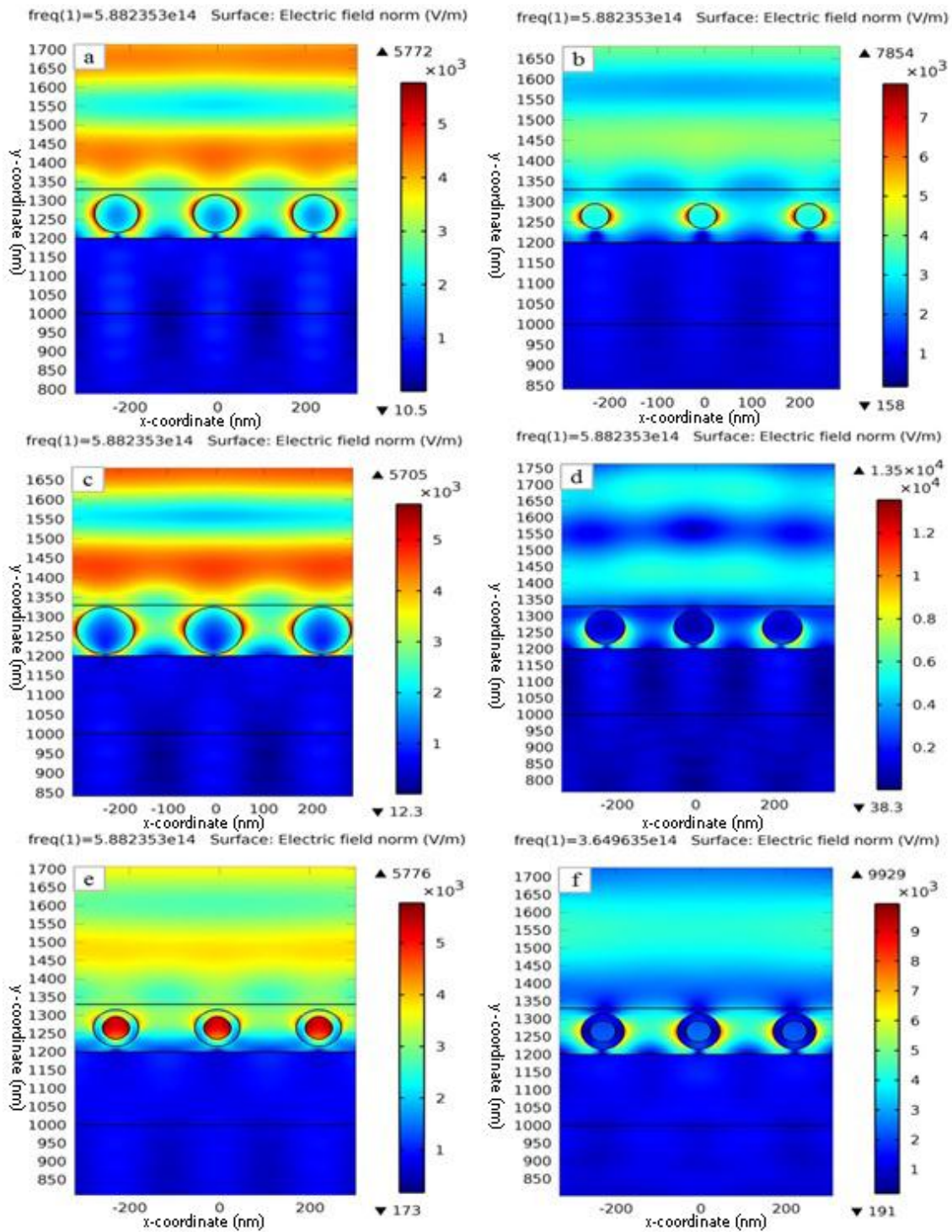
Fig. 3. Influence of NPs plasmonic resonances on light propagation in the structure, (a) NPs radius 50 nm, (b) NPs radius 30 nm and increasing of NPs inter-distance, (c) NPs radius 60 nm and decreasing of NPs inter-distance, (d) NPs material Ag, (e) core/shell NPs at 517 nm, and (f) core/shell NPs at 833 nm.
