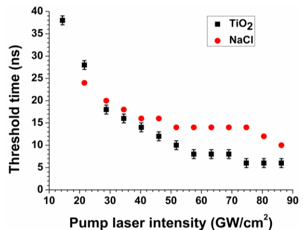
Fig. 5. Threshold time versus pump laser intensity for laser induced breakdown for NaCl in distilled water (circles) and in colloidal \text{TiO}_2 nanoparticles (squares).
