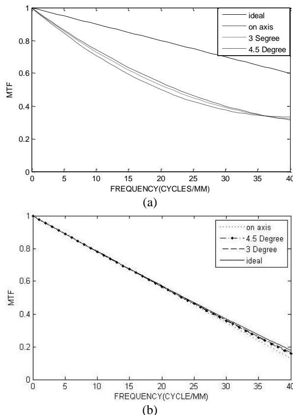
Fig. 7. Modulation transfer function of the optical system with relay lens for ideal case (diffraction limited), on axis (at 0° field of view), 3 and 4.5 degrees fields of view for: a) 3.3 to 5 \mu\text{m} and b) 8 to 12 \mu\text{m} .
