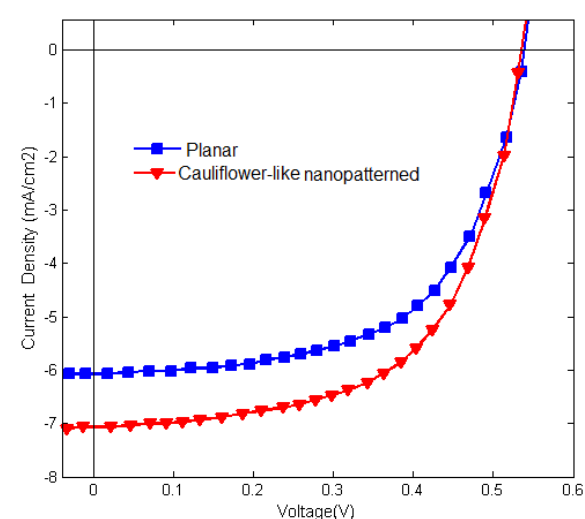
Fig. 5. Current density-voltage (J-V) characteristics of the planar and cauliflower-like nanopatterned back electrode devices measured under AM 1.5 illuminations at 100 mW/cm 2
