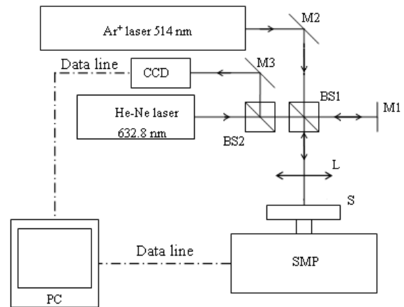
Fig. 1 Experiment setup: pump \text{Ar}^+ laser, probe He-Ne laser, BS-beam splitter, M-mirror, L-Lens, S-sample, SMP-submicropositioner.
