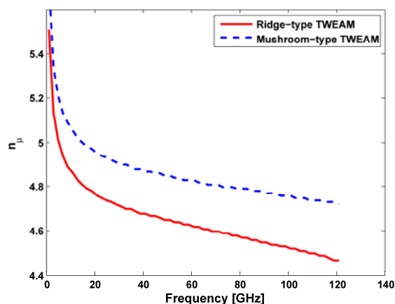
Fig. 11 Microwave refractive index vs. frequency.
