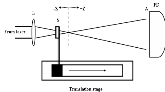
Fig. 1 Open aperture z-scan
