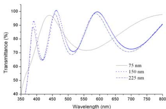
Fig. 4 Transmittance spectra for as-deposited ZnS films at room temperature.
