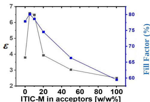
Fig. 9. Comparing simulated \varepsilon with experimental fill factor (FF) vs. weight ratios of ITIC-M in acceptors.
