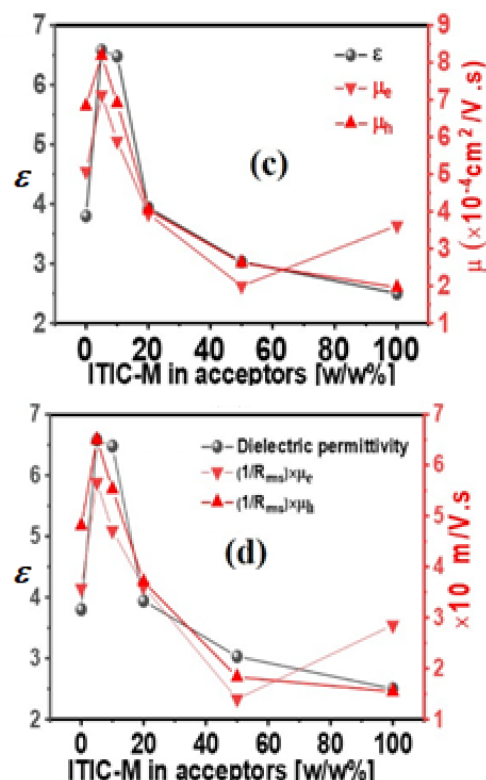
Fig. 10. Comparing simulated \varepsilon with different experimental parameters, including (a) root mean square roughness, (b) carrier lifetime, (c) carrier mobilities, and (d) coupling coefficient of \varepsilon and root mean square roughness vs. weight ratios of ITIC-M in acceptors.
