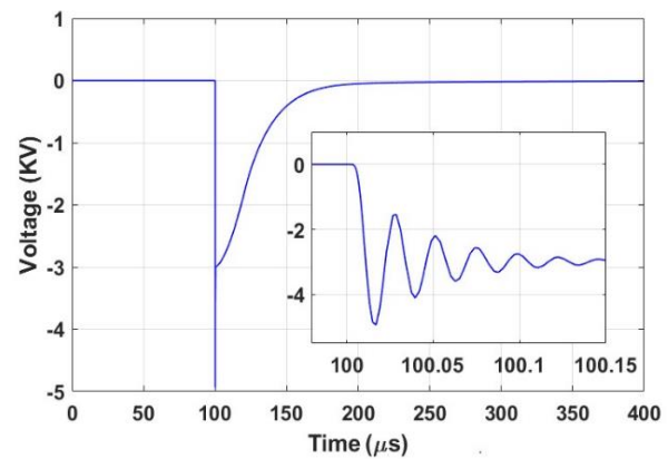
Fig. 6. Voltage overshoot generated at the pulse edge due to LC resonance of the wires and the Pockels cell.
