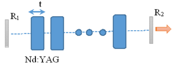
Fig. 4. the implemented model for high average power Nd:YAG ( R_1 and R_2 are the back and output mirror reflectivities)
