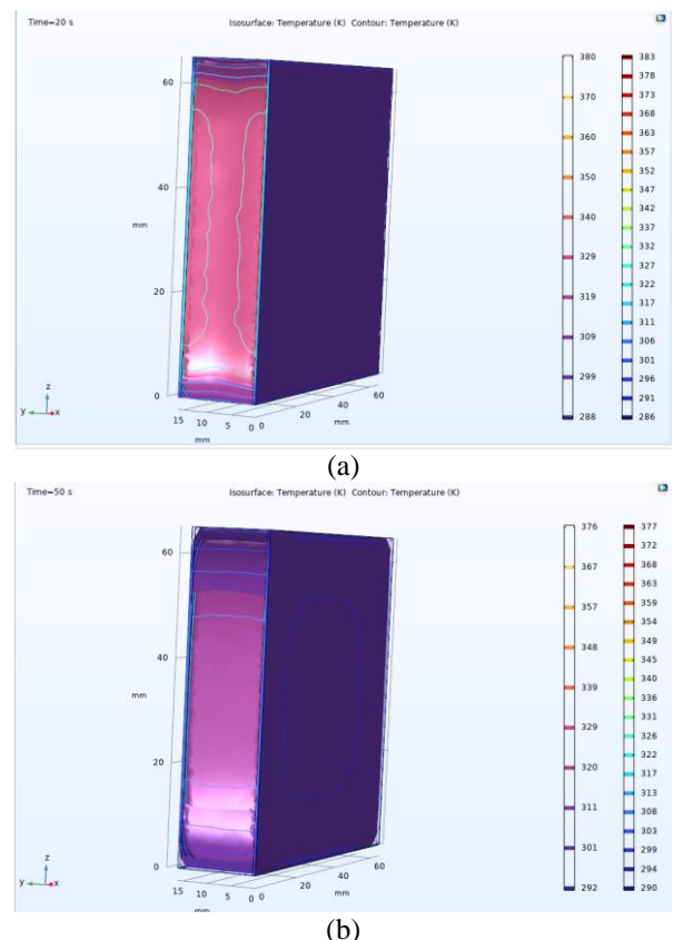
Fig. 12. Cooling phase of the slab by cold air after (a) 20s and (b) 50s.
