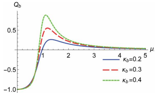
Fig. 4. Mandel parameter for the second mode versus \mu for \kappa_b = 0.2 (solid blue line), \kappa_b = 0.3 (dashed red line), \kappa_b = 0.4 (dotted green line), with N = 10 .
